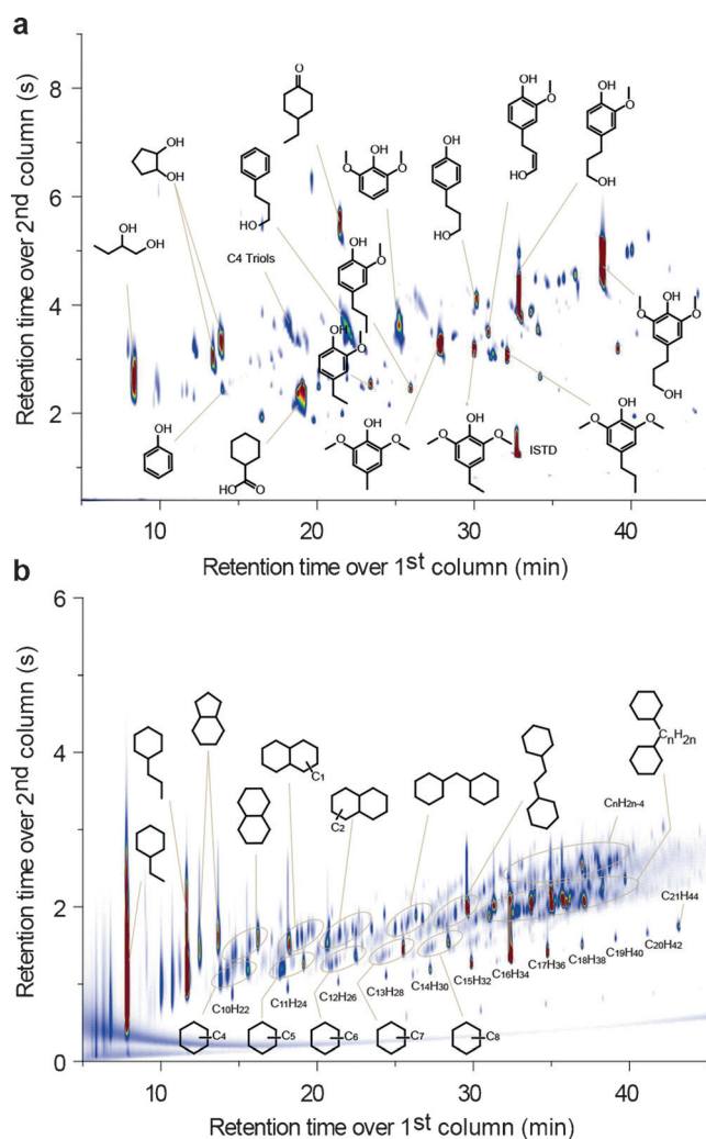
Figure 3. GCxGC-MS analysis of lignin-derived non-pyrolytic bio-oil before (a) and after (b) HDO over PtCo/NOMC-2. Reaction conditions: bio-oil (200 mg), n -hexadecane (GC internal standard, 0.4 mmol), catalyst (200 mg), and n -hexane (solvent, 5 mL), 10 MPa (573 K, constant), 573 K for 12 h.
